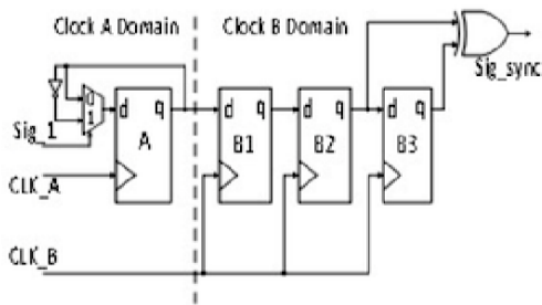
Figure 2: Representing Toggle Synchronizer
