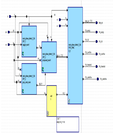
Figure 5: Representing the Proposed block diagram for dual D-FF FIFO Synchronizer.
