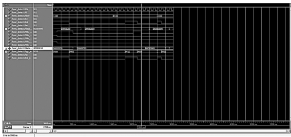
Figure 16: Representing the input observed from the data_in signal for the FIFO sync designed
