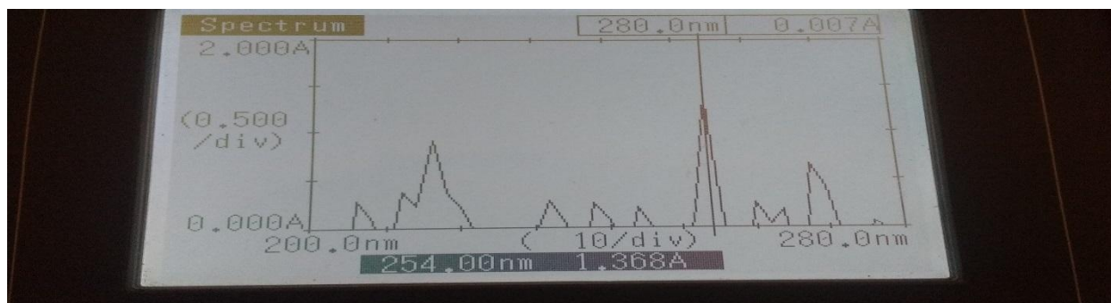
Fig. 1. Peak detection \lambda_{\max} for flurbiprofen in chloroform
