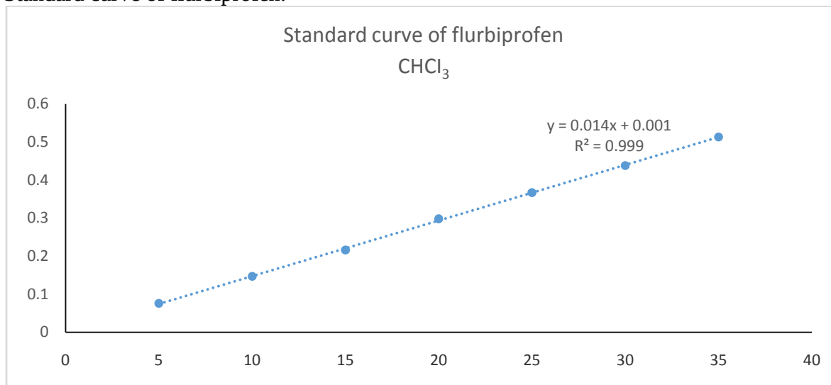
Fig 2. Standard curve calibration of flurbiprofen
