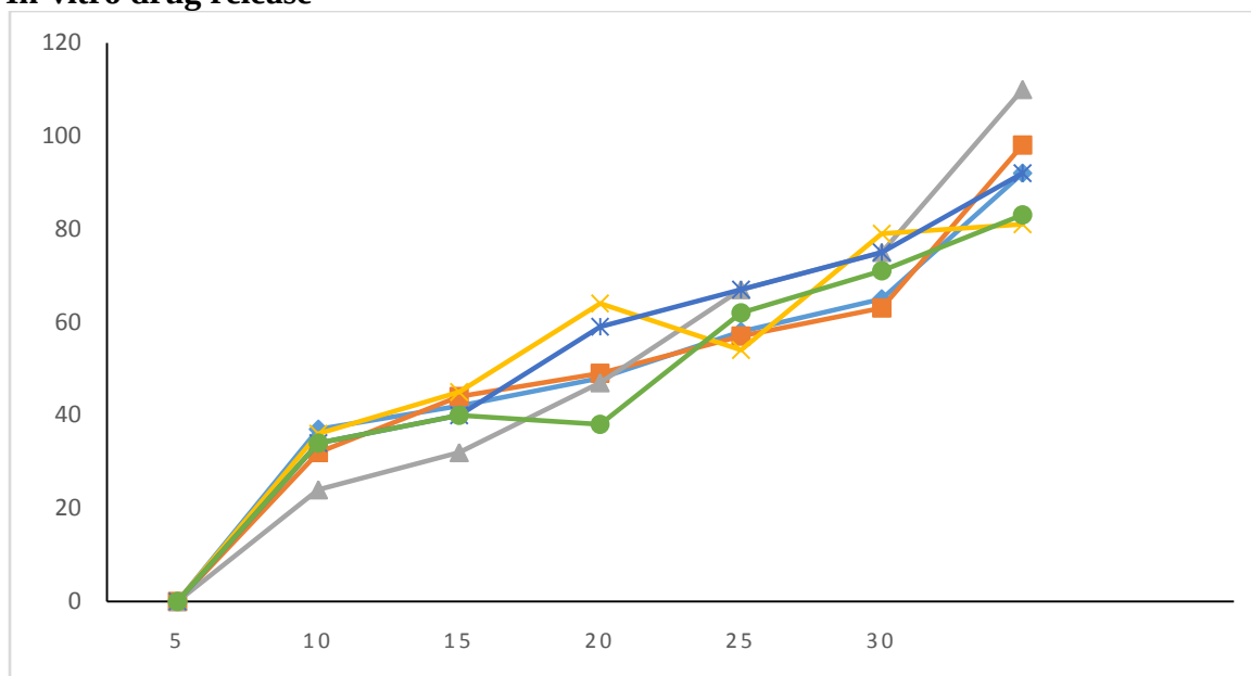
Fig. 4. In-vitro flurbiprofen release
