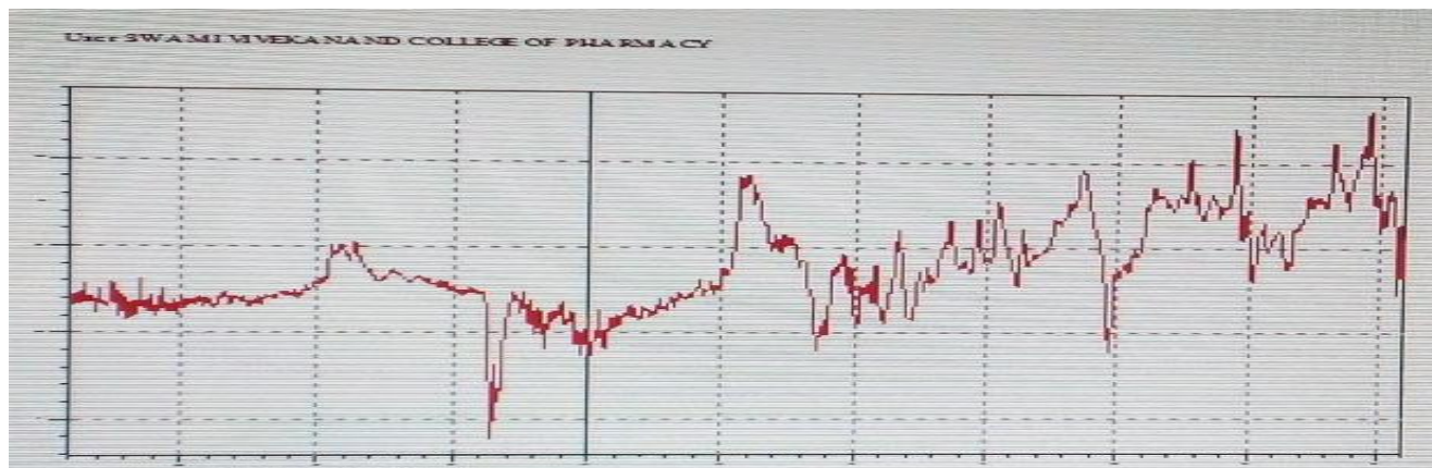
Fig. 3. IR spectrum of flurbiprofen drug sample
